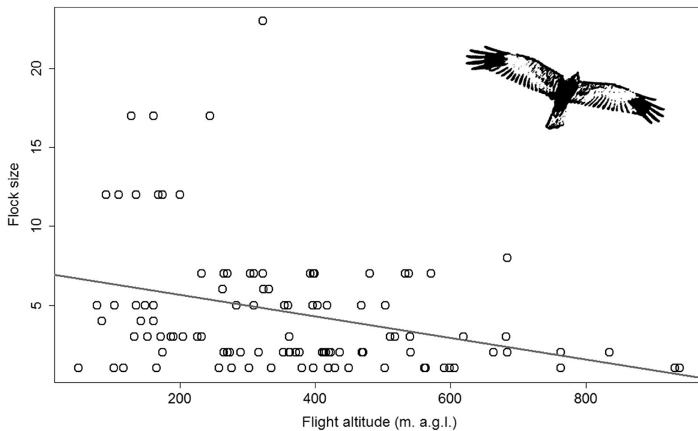
Fig. 3 The relationship between flock size and flight altitude of Western Marsh Harriers
