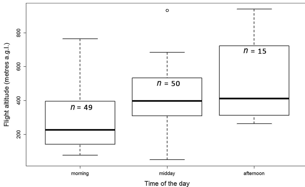
Fig. 4 Flight altitude of Western Marsh Harriers during the day, recorded in 2014 in the Aspromonte mountain (Strait of Messina). The horizontal bold lines show the median flight altitude of each slot. The bottom and top of boxes show the 25 and 75 percentiles, respectively. The horizontal line joined to the box by the dashed line shows the maximum and the minimum range of the data. Points are outliers
